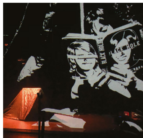
Black Hole
